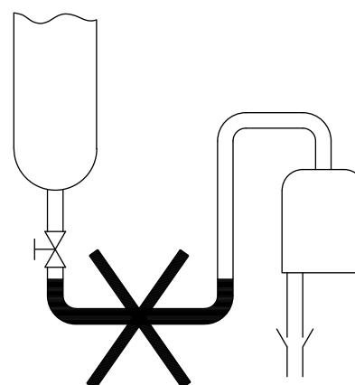
Figure LD-465-5. Do not install a ball float trap above the drip point or put a loop or pocket in the line to the trap. The water seal prevents air from leaving trap body and allowing liquid to enter.
