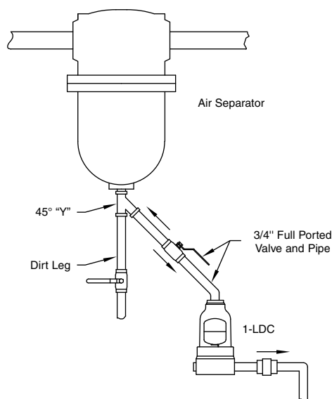
Figure LD-446-1. Typical Drain Trap Location
