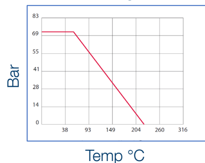
P/T Diagram
